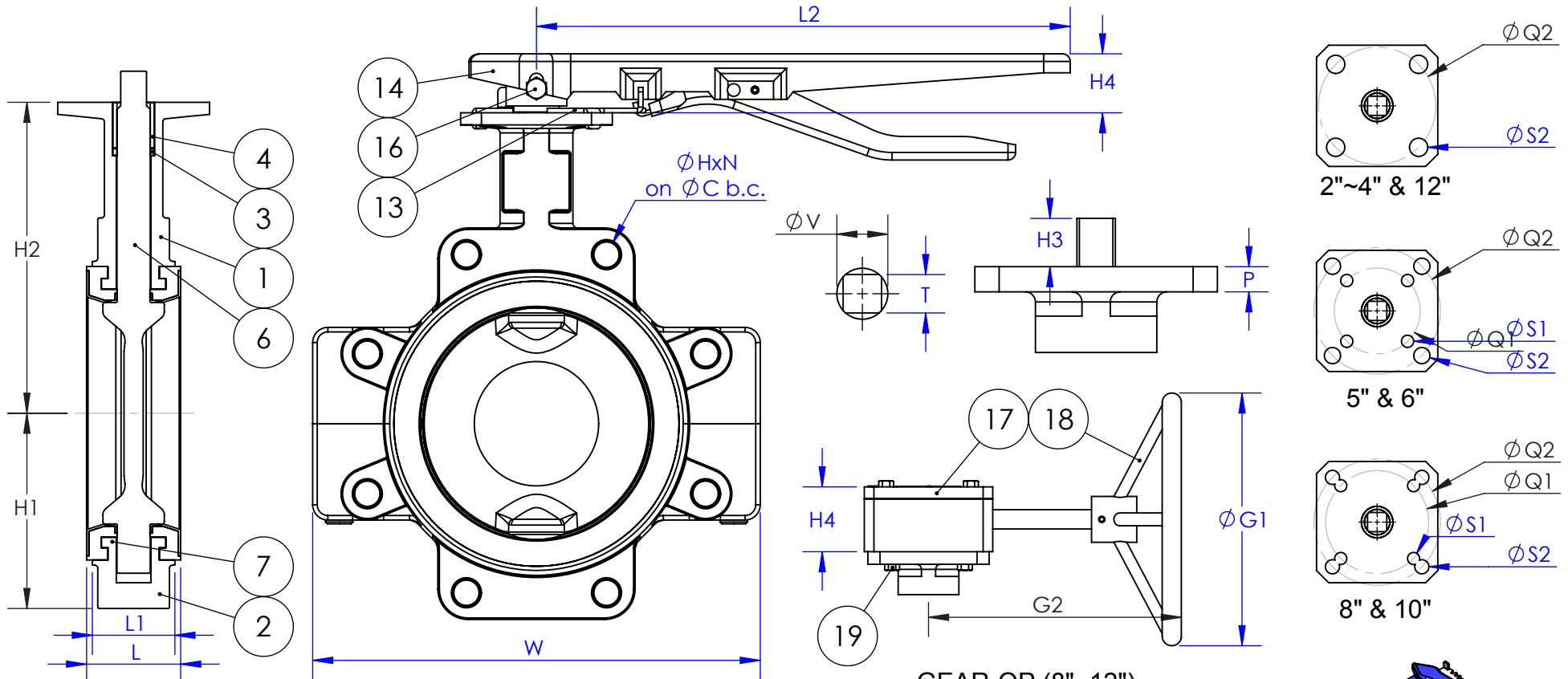
GEAR-OP (8"~12")
